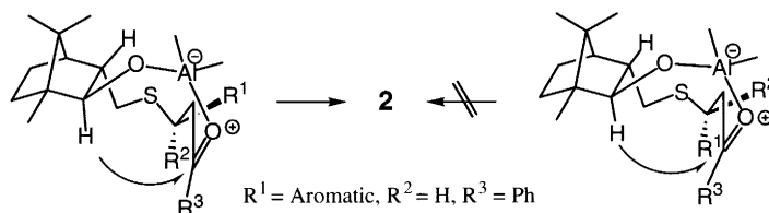
Scheme 3. Plausible transition states for sulfide 2
